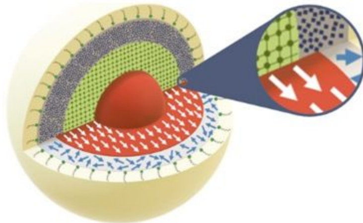
Figure 1: Representation of the structure (vertical cut) and magnetic (horizontal) morphology of Co ferrite NP [3]. Blue arrows indicate surface spin disorder.
