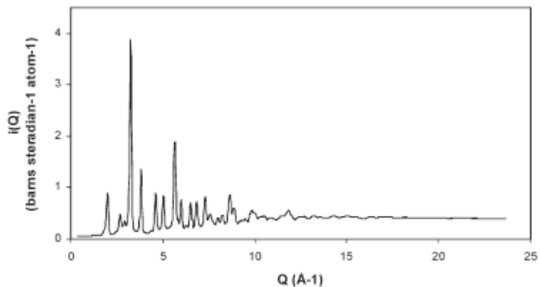
Figure 2. \alpha - U_4O_9 neutron diffraction pattern corrected from air and sample holder diffusion.
